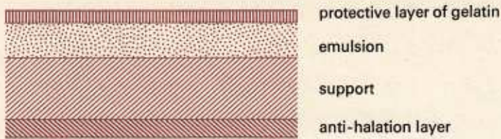
Section through a typical film
