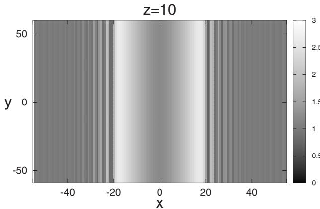
FIG. 16. Density plot of the output intensity evolved from a striplike initial distribution; \gamma=0.1 and output coordinate is equal to z=10 .
