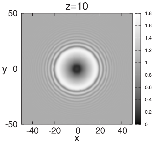
FIG. 17. Density plot of the output intensity evolved from a circle initial distribution; \gamma=0.1 and output coordinate is equal to z=10 .
